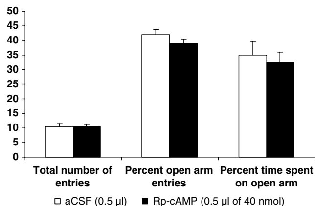
Figure 11 Effect of NAc shell infusion (3 days of once daily) of aCSF and PKA inhibitor (Rp-cAMP) on open- and closed-arm activities of the elevated plus maze as a measure of anxiety-like behaviors. Values are the mean \pm SEM of 11–13 rats in each group.
